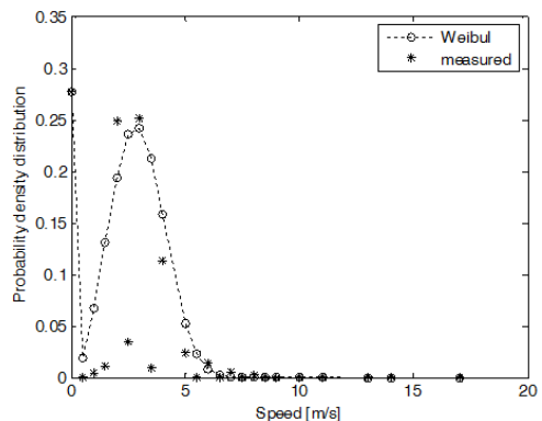
Figure 5: Wind speed frequency distribution for Gisenyi station
