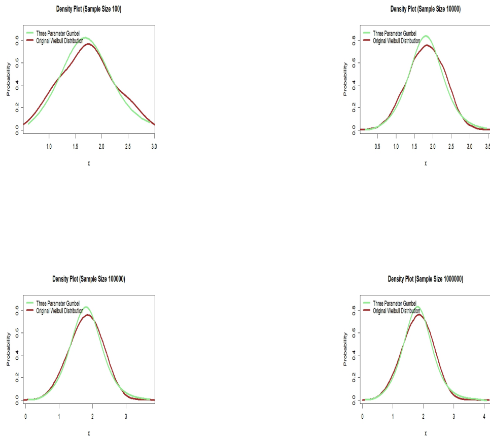
Fig. 10. Asymptotic distributions for three parameters Gumbel and Weibull distributions
