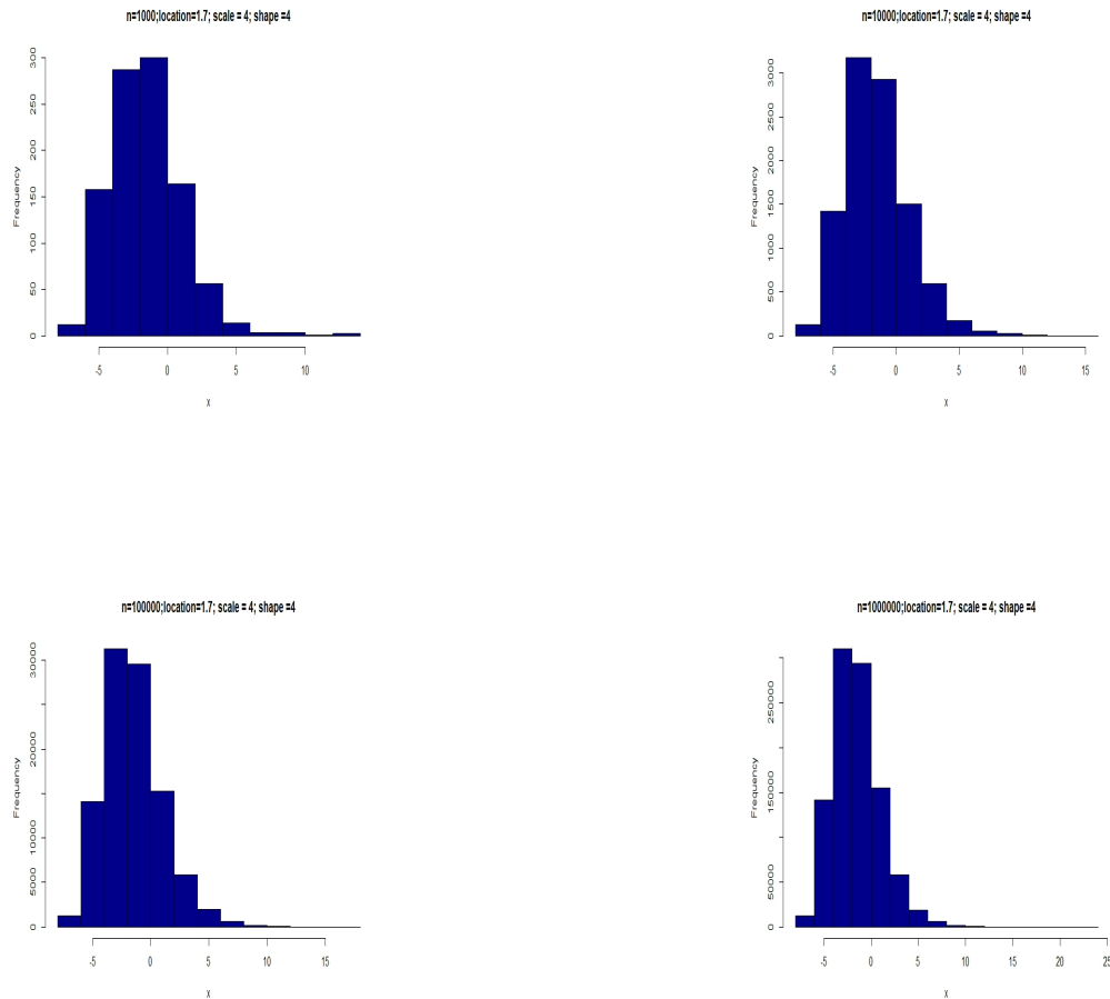
Fig. 4. Distributions when \omega, \tau and \delta are constant and n is varying
