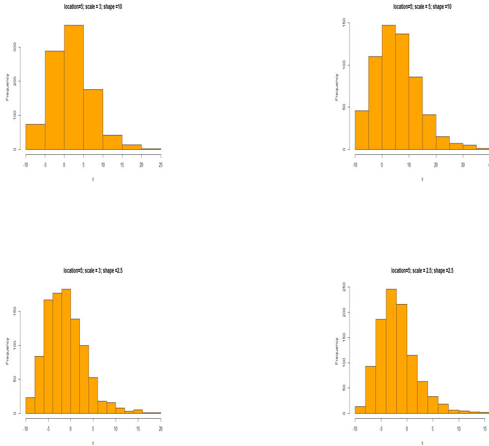
Fig. 1. Distributions when \omega and n are constant
