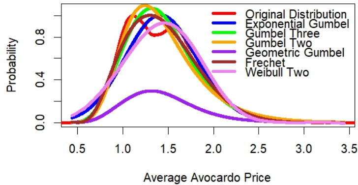
Fig. 12. Data 2: Avocado prices in dollars
