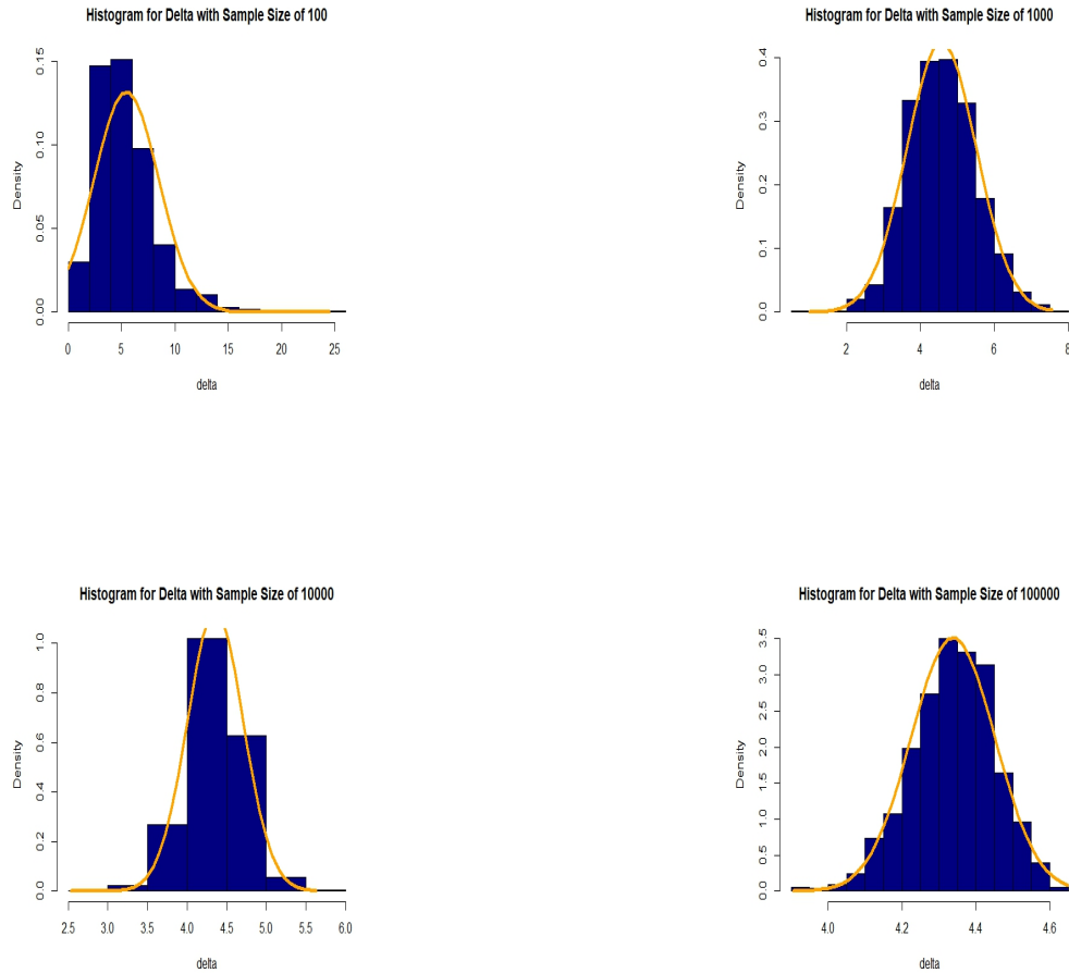
Fig.6. Asymptotic distributions for \delta
