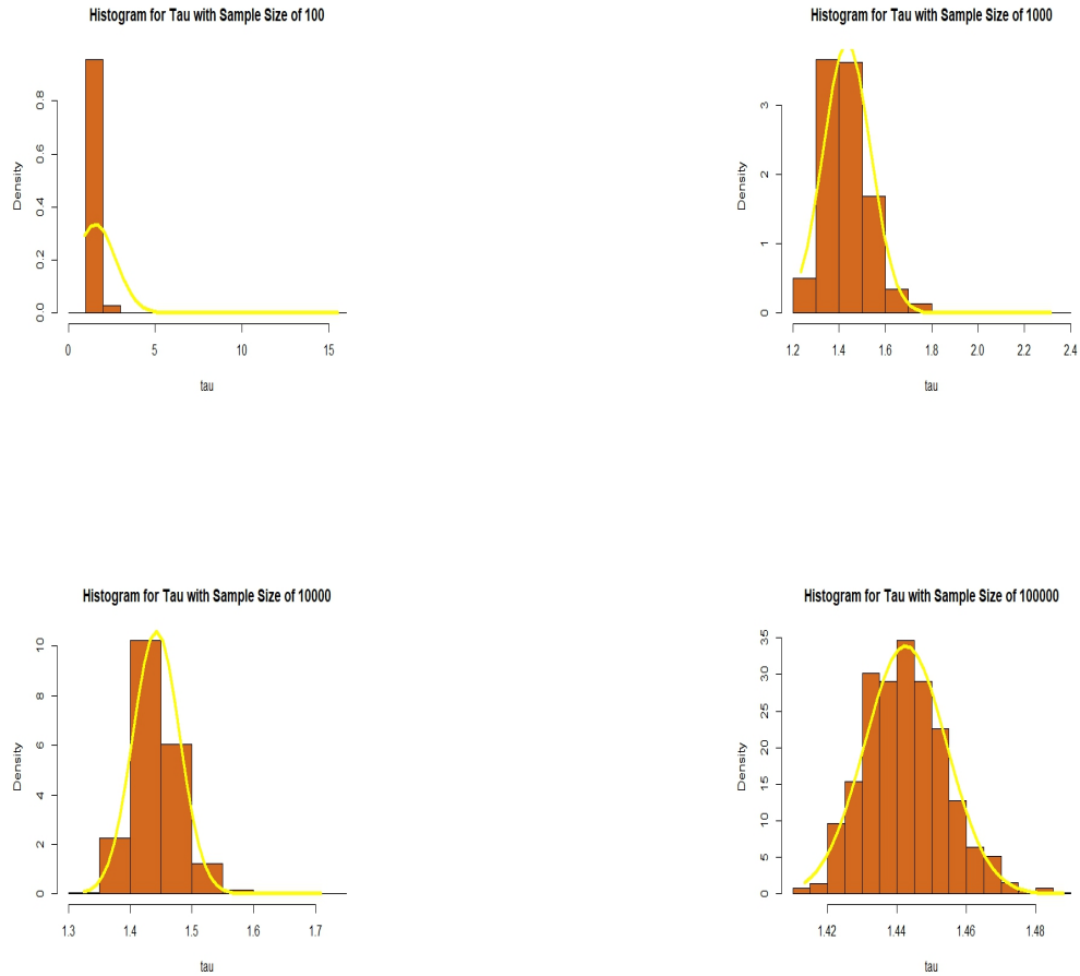
Fig. 7. Asymptotic distributions for \tau
