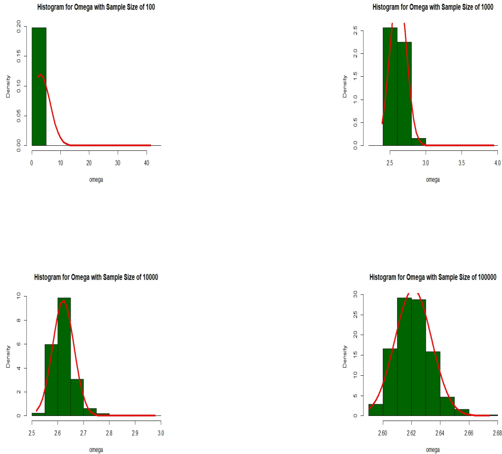
Fig. 5. Asymptotic distributions for \omega
