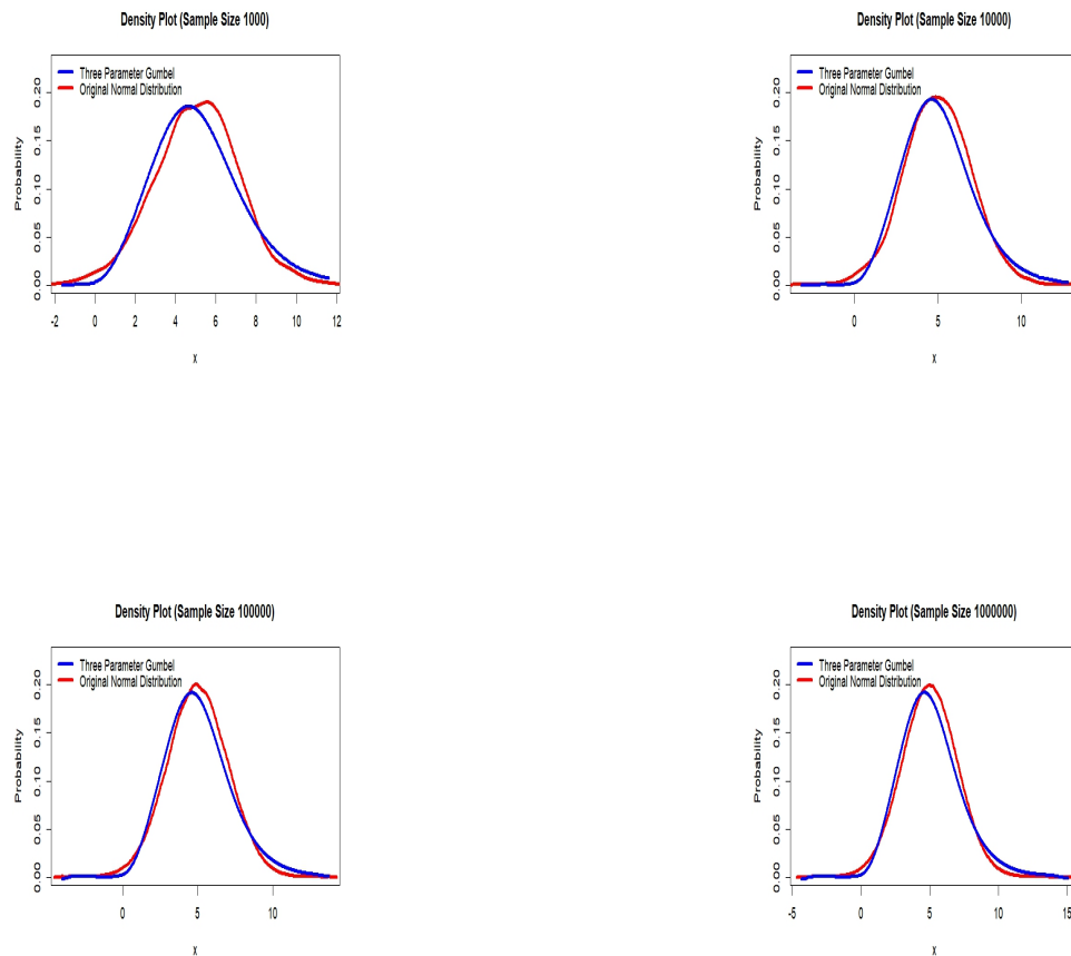
Fig. 8. Asymptotic distributions for three parameters Gumbel and normal distributions
