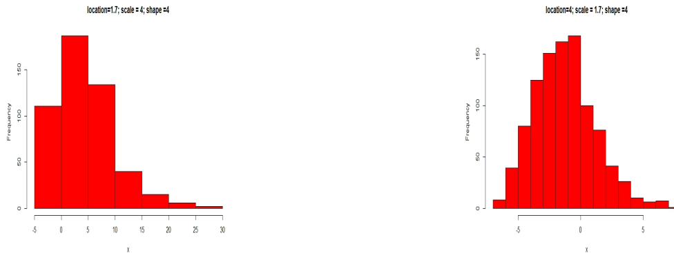
Fig. 3. Distributions when \delta are n are constant
