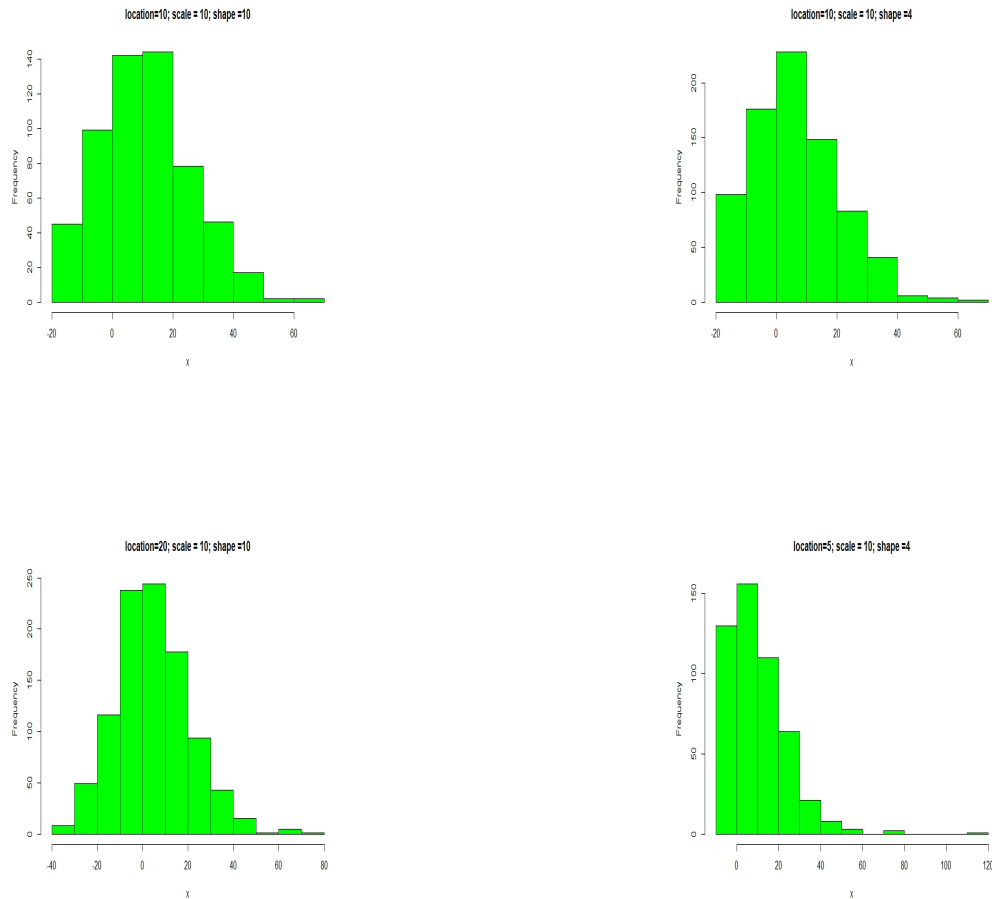
Fig. 2. Distributions when \tau and n are constant
