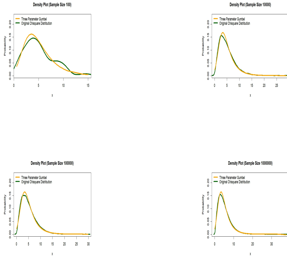
Fig. 9. Asymptotic distributions for three parameters Gumbel and chi-square distributions
