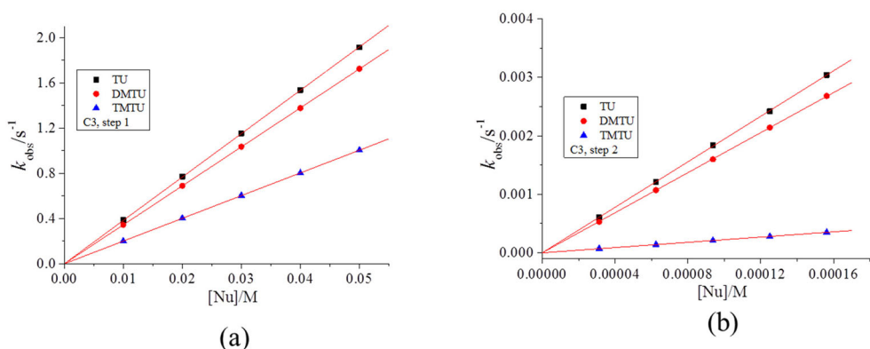
Figure 4. Plots of k_{\text{obs}} (a) and k_{\text{obs}'} (b) vs. [Nu] for the reactions of 3 with the thiourea nucleophiles at 298 K.
